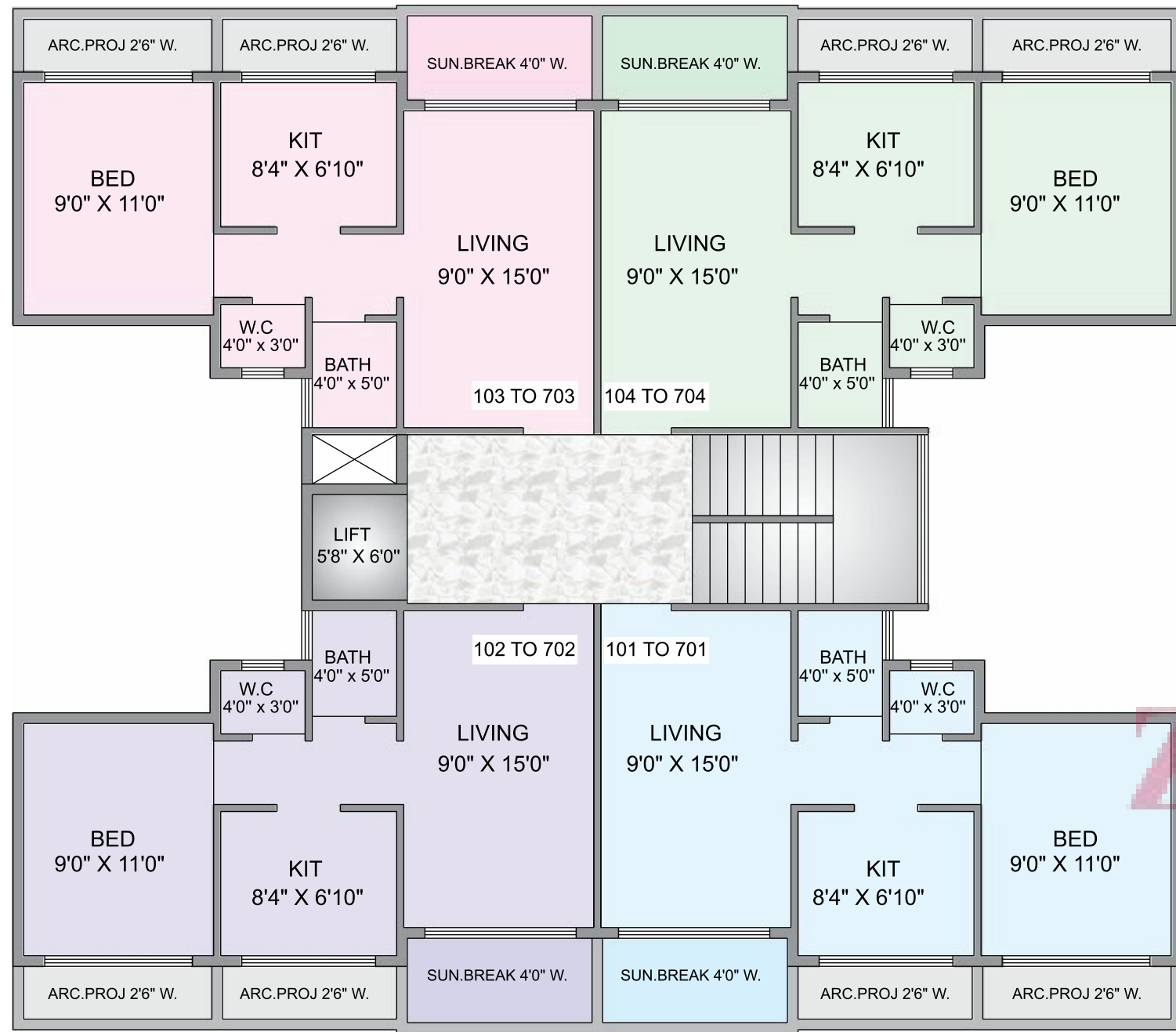
1ST TO 7TH FLOOR PLAN FOR ( WING 'R-3')
